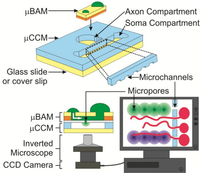
Figure 1. Illustration of modular microfluidic system that enables flexible user-defined chemical gradient presentation for axonal guidance studies.
